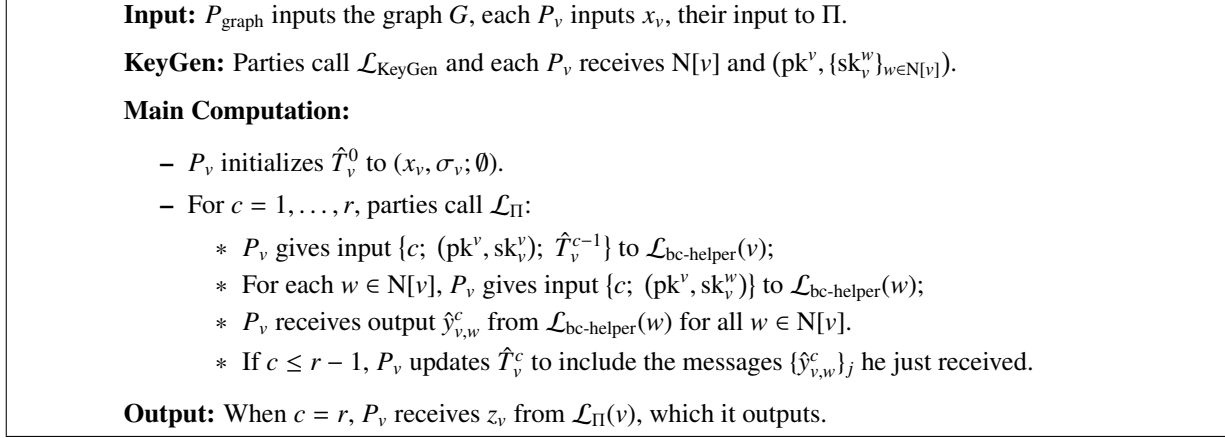
Figure 8: The (\mathcal{L}_{\text{KeyGen}} \parallel \mathcal{L}_{\Pi}) -hybrid protocol \Pi' .
