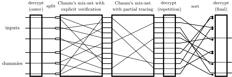
Fig. 1. Execution of Protocol 4 with N = 3 senders, k = 3 mix-servers, and t = 2 repetitions, where all parties are honest. Each party submits a bundle of two ciphertexts containing identical innermost ciphertexts. The bundle is decrypted and split into two ciphertexts. All ciphertexts are then individually shuffled in the two instances of Chaum’s mix-net. Then the first is verified explicitly (revealing the permutation), the dummy ciphertexts are traced in the second (revealing the paths of the dummies) and the output is decrypted and verified to contain t copies of each ciphertext. If all tests passed, then a final round of decryption recovers the plaintexts.
